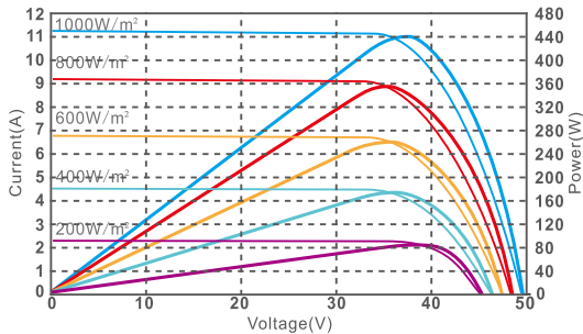
I-V characteristics at different irradiances
