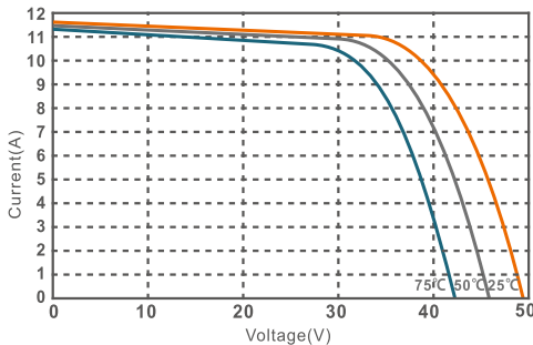
I-V characteristics at different temperature
